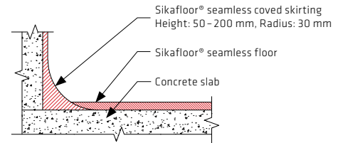
Coved skirting applied before floor covering
