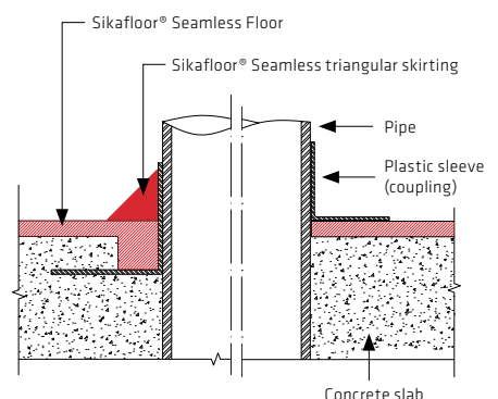
Connections to pipes
