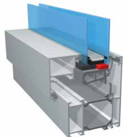
Glass Edge Bonding with Sikasil® WT Technology
