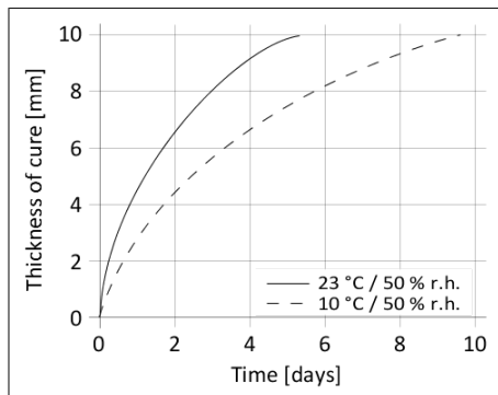
Diagram 1: Herdehastighet for Sikaflex®-298 FC
