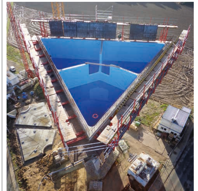
Water tower Beersel, Belgium: Sikaplan® WT-4220.
