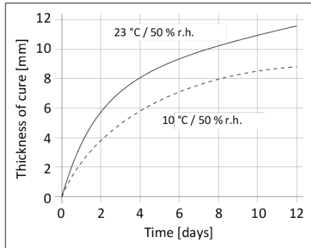
Diagram 1: Herdehastighet SikaTack® MOVE Global 30
