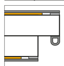
Frame and cover bonding Sikaflex®-221/-553, Sikasil® SG-500/SG-20
