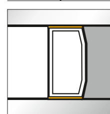
IG primary sealing SikaGlaze® IG-5 PIB
