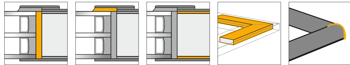
Burglary protection Sikasil® WT-480
