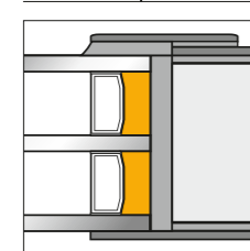
IG secondary sealing Sikasil® IG-25 HM Plus
