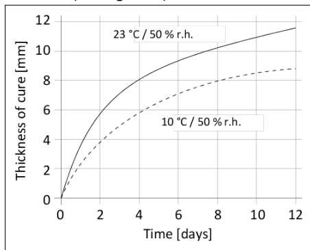
Diagram 1: Herdehastighet SikaTack® MOVE Global 30
