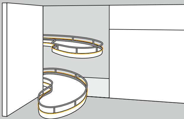
Metal rails bonded to wood base with SikaFast®-5215 NT .
